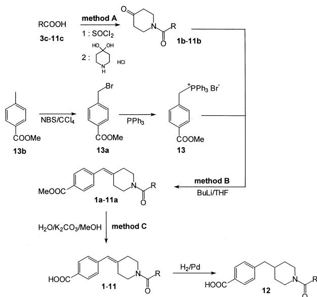
Scheme 2. Synthetic strategy.
